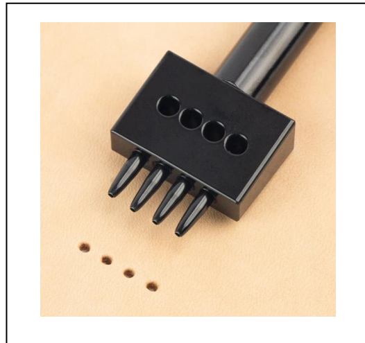
Hole Punch Round_4 Prongs - 1mm
